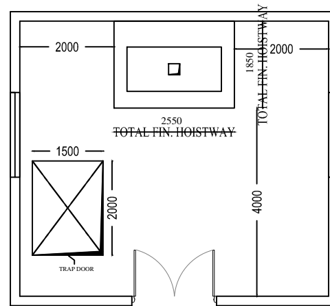
MACHINE-ROOM PLAN
