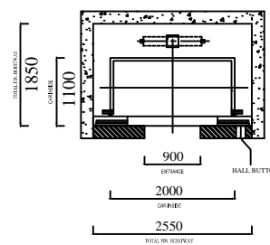
HOISTWAY PLAN
